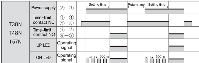
■ C type (Time - limit 2c)
