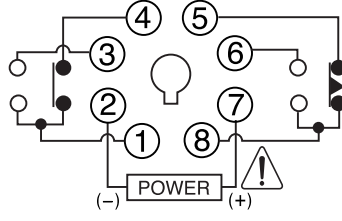
■ B type (Time - limit 1c + Instantaneous 1c)
