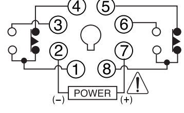
■ F type (Time - limit 2c)
