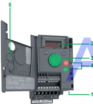
ATV310H037N4E with door on front panel open
