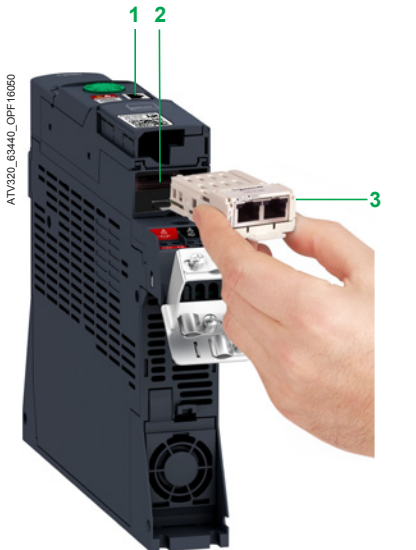
Example of installing a communication module 3 (view of underside)
