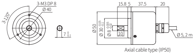
Axial cable type (IP50)
