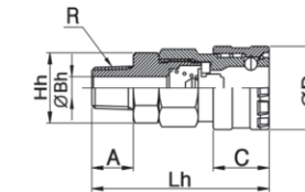
MODEL [ØD-T] Tube (Metric) – Thread (R)
